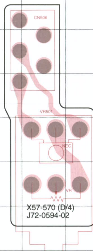
VOL, ENC UNIT (X57-570X-XX) (D/4) Component Side View + Foil Side View
