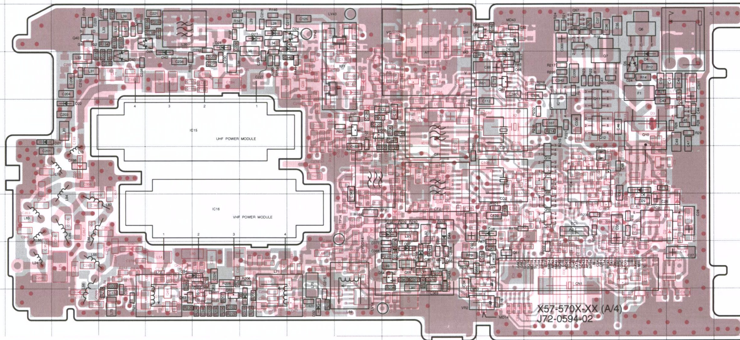
RF UNIT (X57-570X-XX) (A/4) Component Side View + Foil Side View
