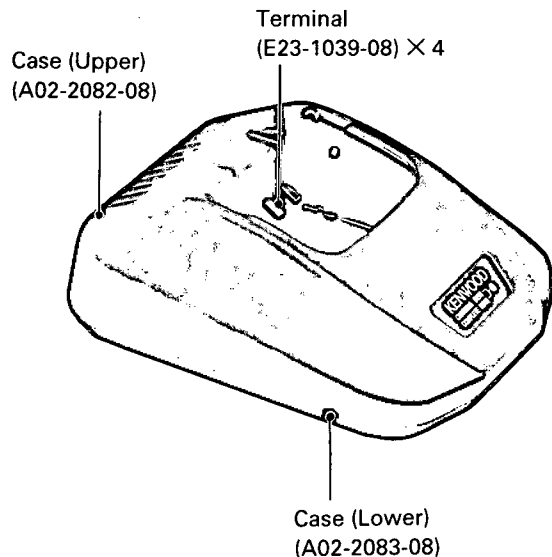
BC-19: External view
