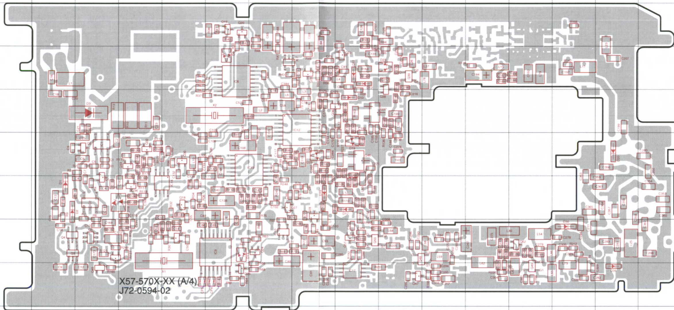
RF UNIT (X57-570X-XX) (A/4) Foil Side View
