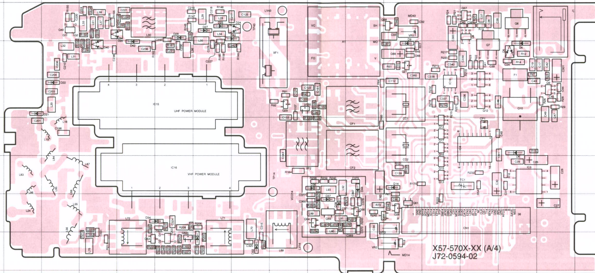
RF UNIT (X57-570X-XX) (A/4) Component Side View
