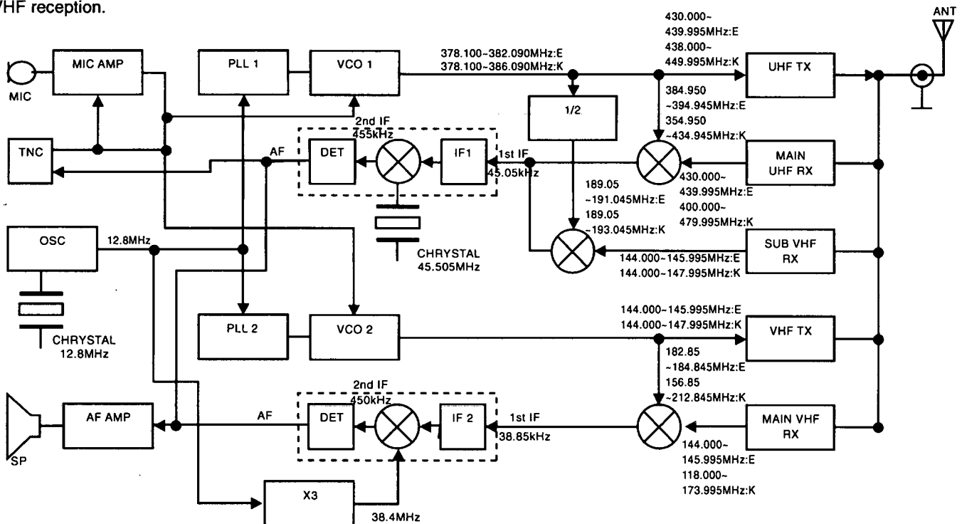
Fig.1 Frequency Configuration
