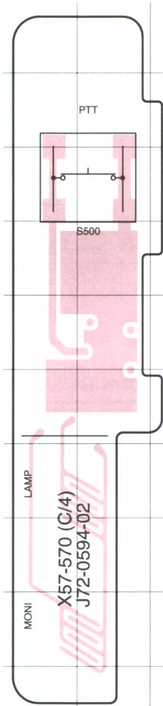
PTT UNIT (X57-570X-XX) (C/4) Component Side View
