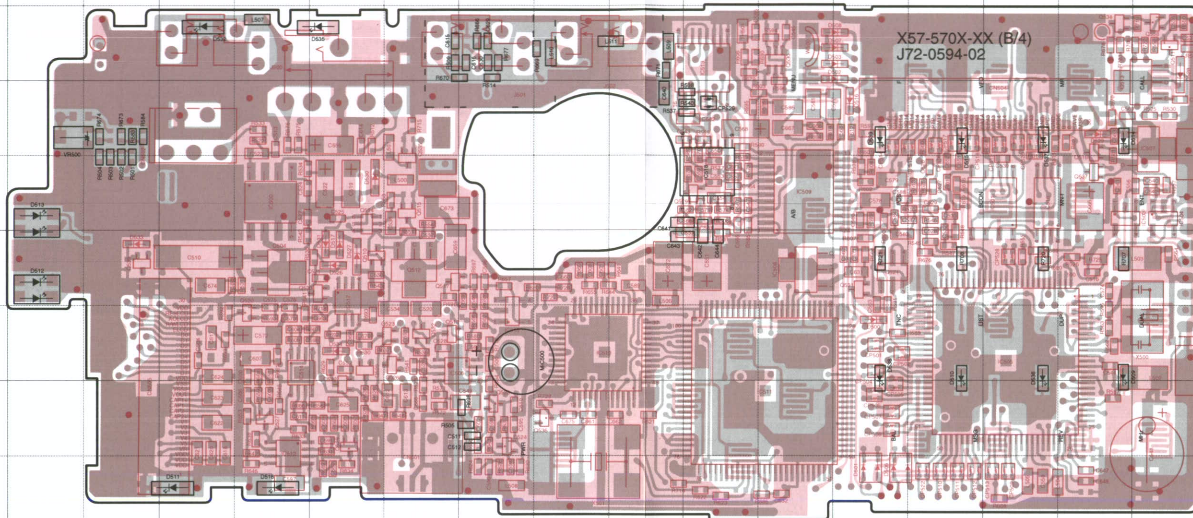
CONTROL UNIT (X57-570X-XX) (B/4) Component Side View + Foil Side View
