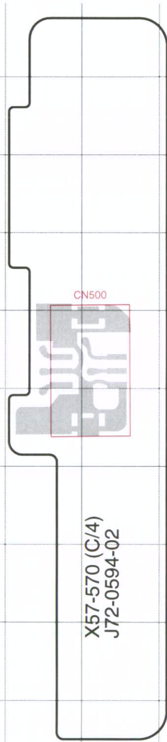
PTT UNIT (X57-570X-XX) (C/4) Foil Side View
