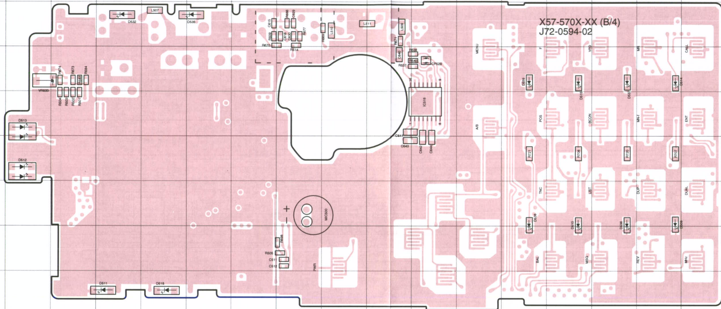
CONTROL UNIT (X57-570X-XX) (B/4) Component Side View
